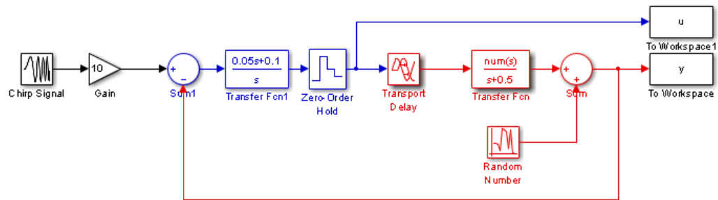
Red part: system to be modeled using IDPROC Blue part: Controller
