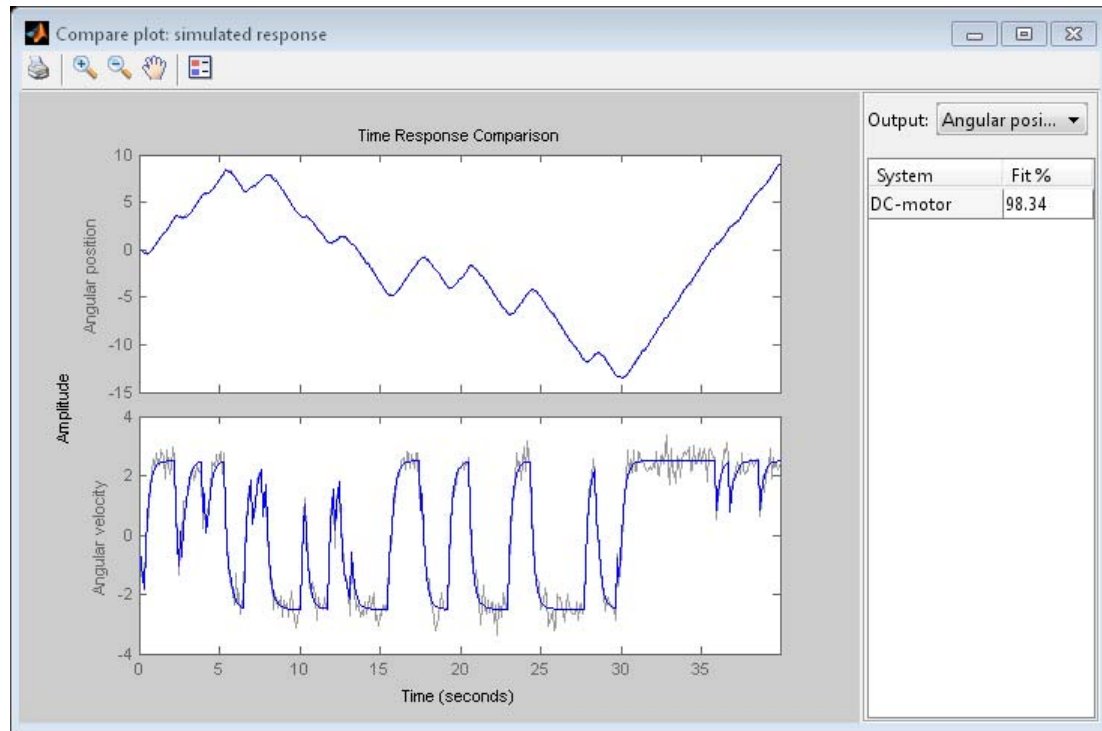
Figure 4: Comparison between measured outputs and the simulated outputs of the estimated IDNLGREY DC-motor model.
