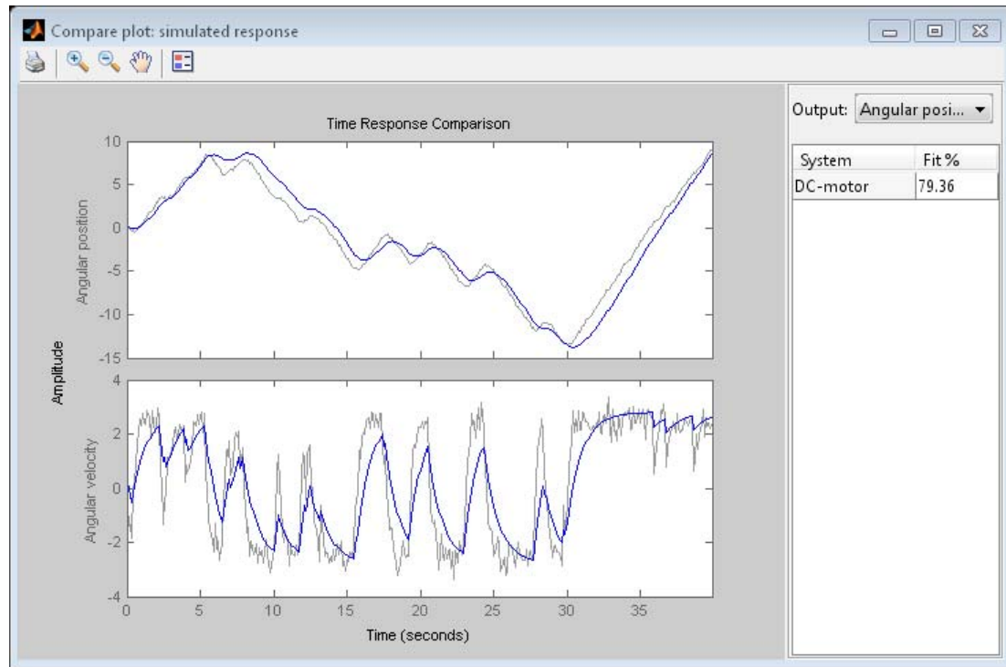
Figure 3: Comparison between measured outputs and the simulated outputs of the initial DC-motor model.
