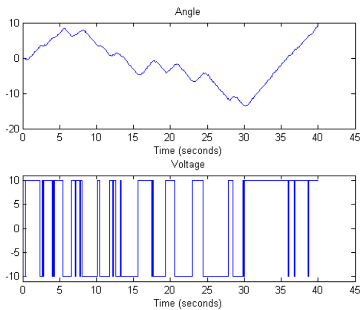
Figure: Measurement Data: Voltage to Angle
