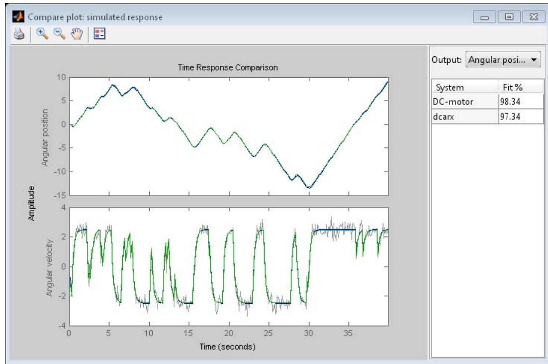
Figure 5: Comparison between measured outputs and the simulated outputs of the estimated IDNLGREY and ARX DC-motor models.
