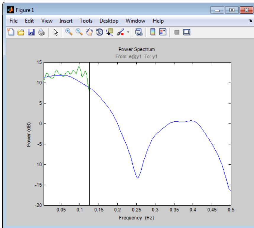
Folding Effects with Manual Decimation
